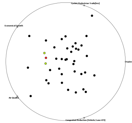
Figure 5: A RadViz application [8] of the transportation asset management problem. The colored points demonstrate a drawback of RadViz, as it does not support the adjacency requirement. Specifically, non-similar solutions can be placed close to each other.
