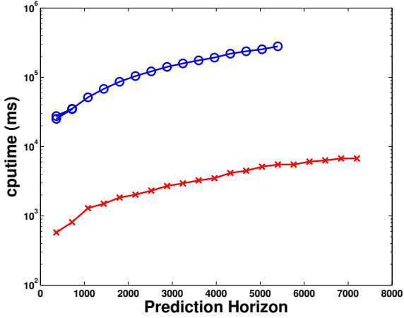
Fig. 3. Runtime: comparison of scalability between the nonlinear programming control formulation (blue circles) and our proposed decomposition method (red crosses).
