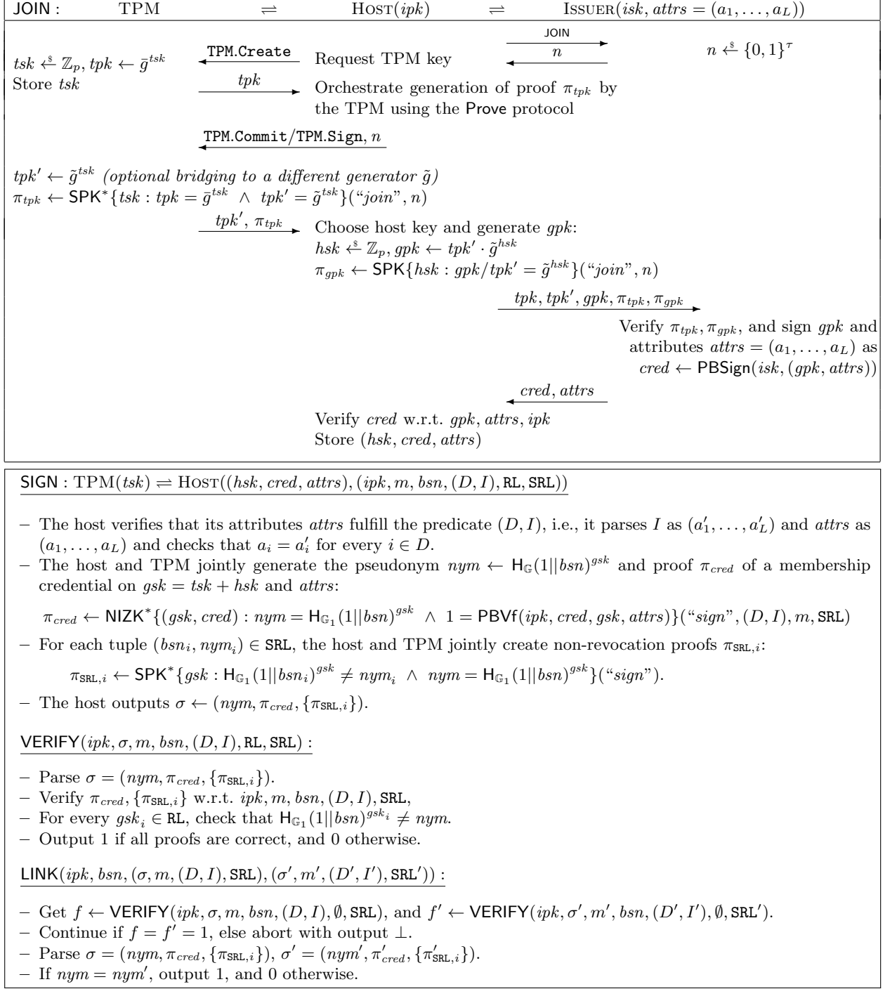
Fig. 4. High-level overview of the DAA protocols.
