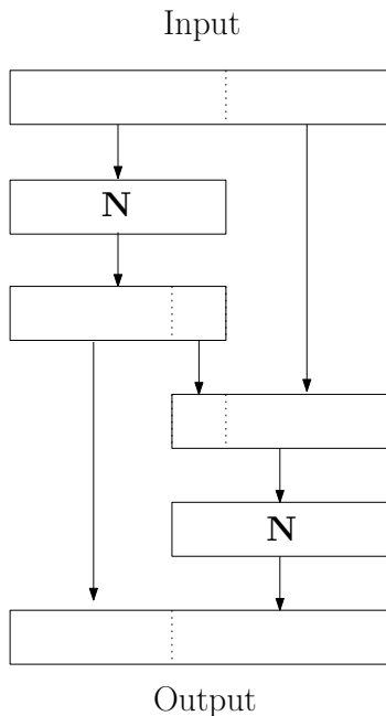
Figure 3: The composite linear transformation \overline{\mathbf{N}}
