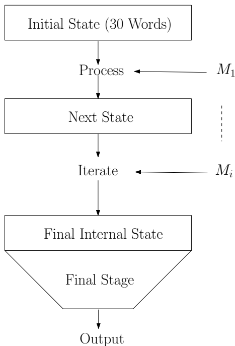
Figure 1: Fugue-256 Structure
