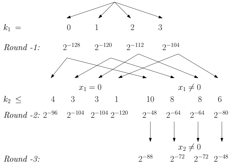
Figure 9: Case Analysis for wF-256
