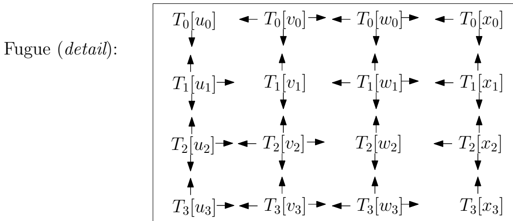
Figure 4: AES Column Mix vs. Fugue Super-Mix
